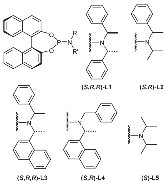
Figure 1. Phosphoramidite ligands.
